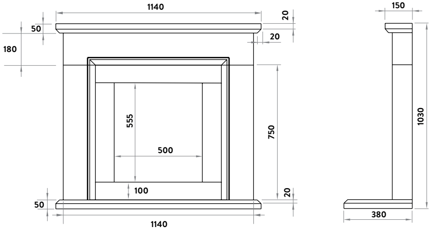
Inspire 400/500 Vicenza Suite Note: When fitting an Inspire 400 model with the Vicenza suite the fireplace opening dimensions are: H: 555 W:400
