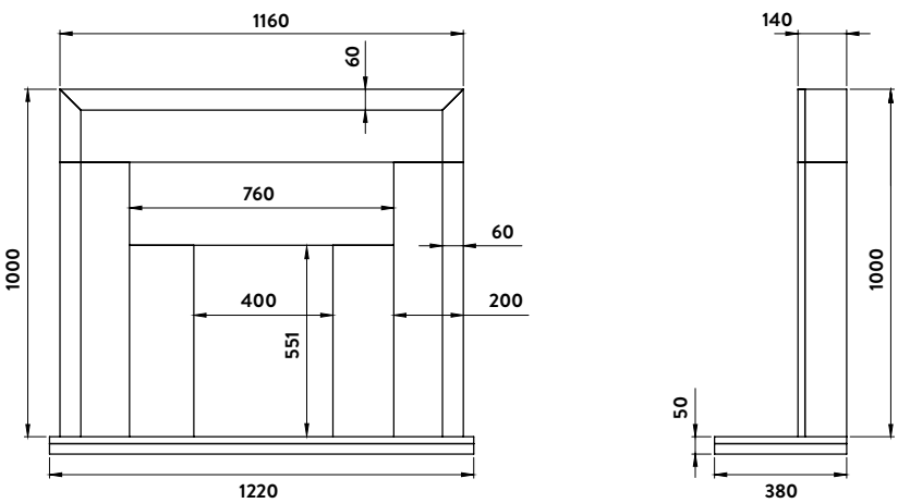
Inspire 400 Atalanta Suite Note: The Inspire 400 gas fire can only be hearth mounted with the Atalanta suite
