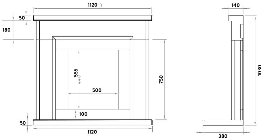
Inspire 400/500 Palermo Suite Note: When fitting an Inspire 400 model with the Palermo suite the fireplace opening dimensions are: H: 555 W:400
